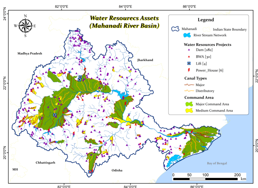
Figure 12 Major Infrastructure of the Mahanadi River Basin
