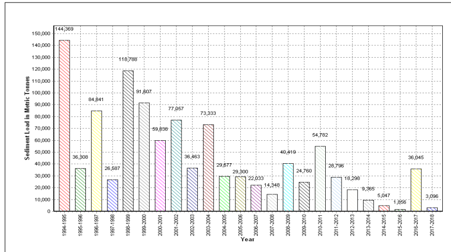
Annual Sediment Load: 1994-2018
