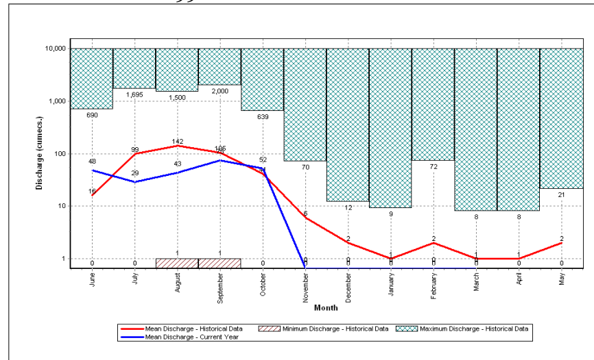
Histogram Hydrograph for the Water Year 2017-18
