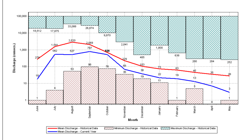
Histogram Hydrograph for the Water Year 2017-18
