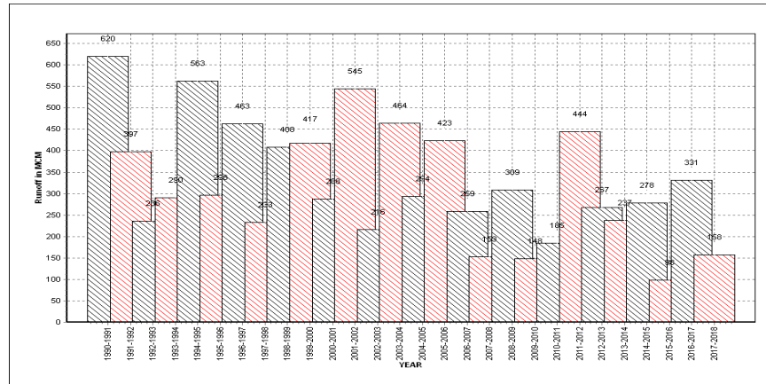
Annual Runoff Values between 1990-2018
