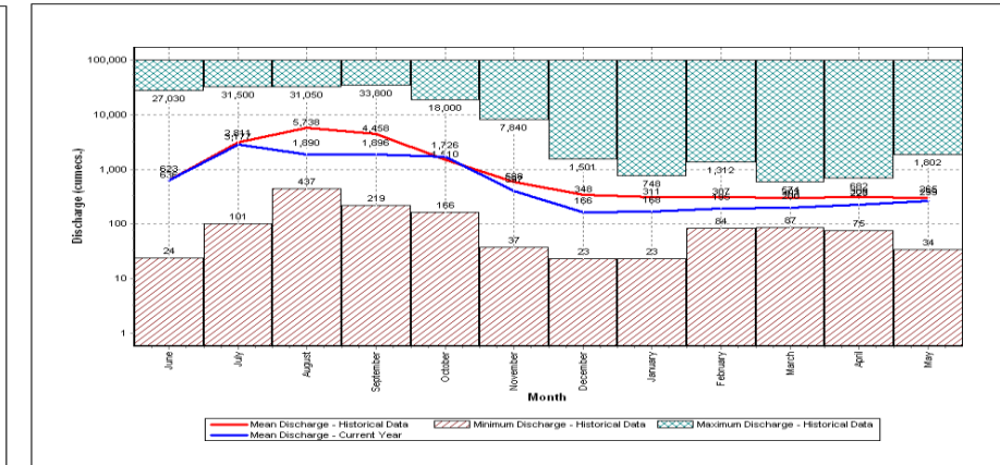
Histogram Hydrograph for the Water Year 2017-18
