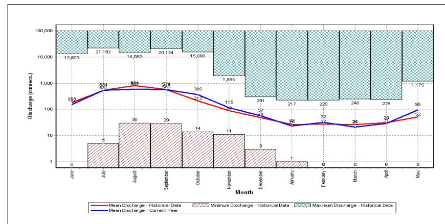
Histogram Hydrograph for the Water Year 2017-2018
